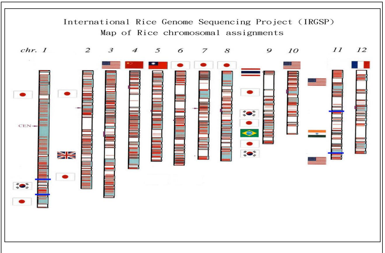
International Rice Genome Sequencing Project(IRGSP)
